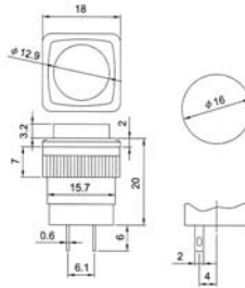
JS-708 A:(ON)-OFF B:ON-(OFF) AL:W/LED(ON)-OFF BL:W/LED ON-OFF
