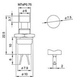
JS-724 A:(ON)-OFF B:ON-(OFF) C:ON-(OFF)
