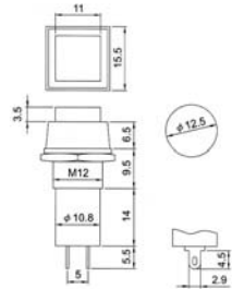
JS-724 A:(ON)-OFF B:ON-(OFF) C:ON-(OFF)
