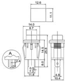
JS-756 A:(ON)-OFF With Separator B:(ON)-OFF W/O Separator
