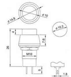
JS-723S A:(ON)-OFF B:ON-(OFF)
