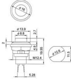
JS-708 A:(ON)-OFF B:ON-(OFF) AL:W/LED(ON)-OFF BL:W/LED ON-OFF
