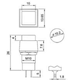
JS-725 A:(ON)-OFF B:ON-(OFF) C:ON-(OFF)
