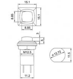
JS-722S A:(ON)-OFF B:ON-(OFF)
