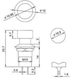
JS-756 A:(ON)-OFF With Separator B:(ON)-OFF W/O Separator
