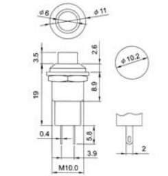
JS-725 A:(ON)-OFF B:ON-(OFF) C:ON-(OFF)
